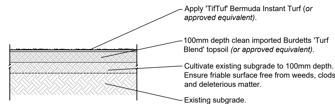
3 Instant Turf Typical Planting Detail Not to scale
