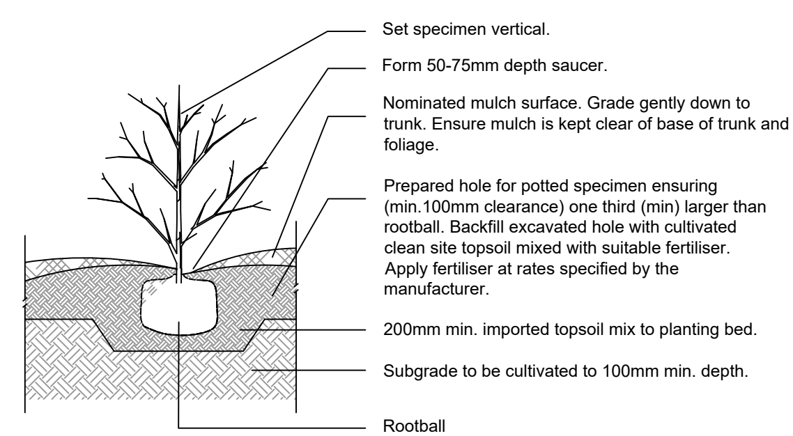
2 Potted Plant Typical Planting Detail 1:20 @ A1
